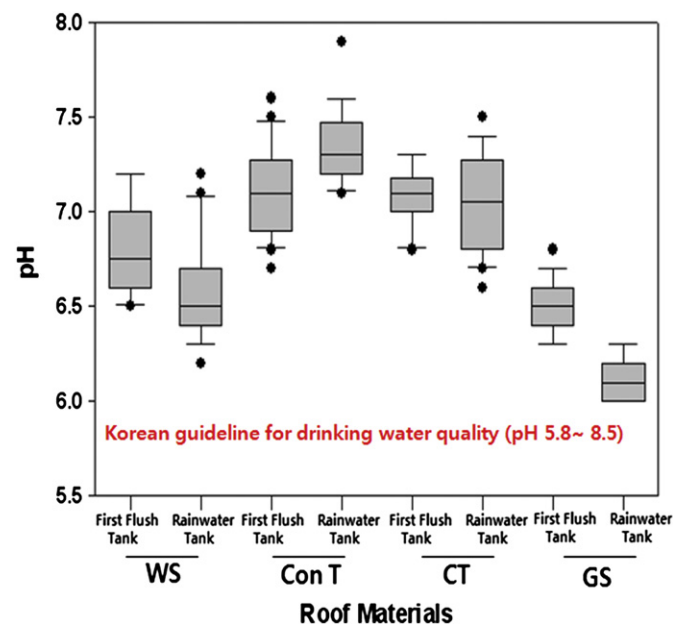
Fig. 2. Box plot diagram of the pH values of rainwater harvested from the four roofing materials (total events [ n = 40 ]). Note: WS = Wooden Shingle; Con T = Concrete Tile; CT = Clay Tile (Gi-Wa); GS = Galvanized Steel.
