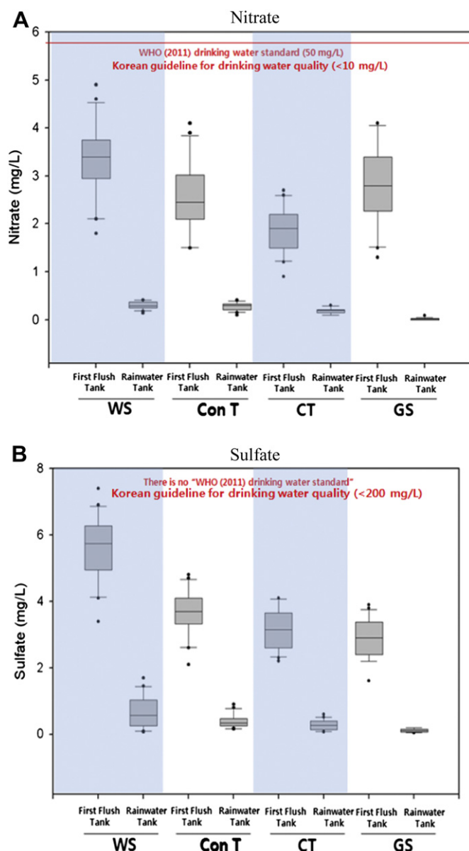
Fig. 5. Box plot diagram for the nitrate ( \text{NO}_3^- ) and sulfate ( \text{SO}_4^{2-} ) concentrations in the water collected from the different roofing materials (total events [ n = 40 ]).
