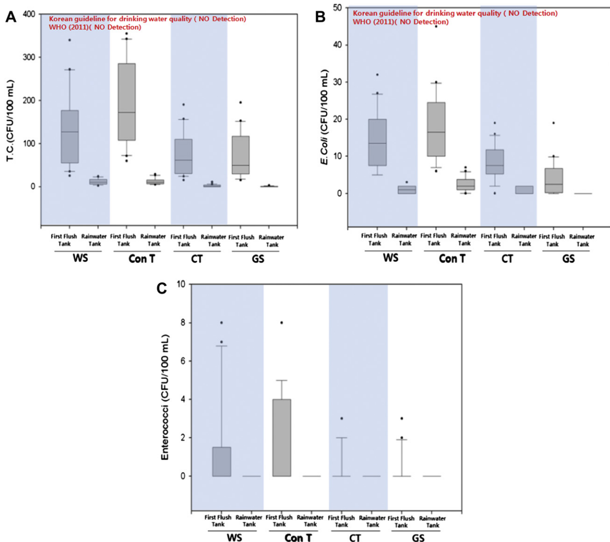
Fig. 7. Box plot diagram for the fecal indicators (total coliform, E. coli , enterococci) identified in the different roofing material samples (total events [ n = 40 ]).
